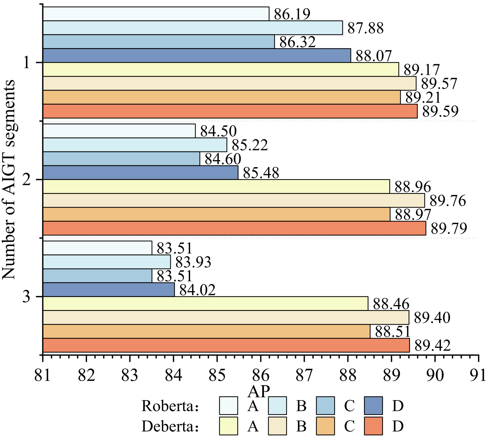
AP based on GPT-Neo generated text
